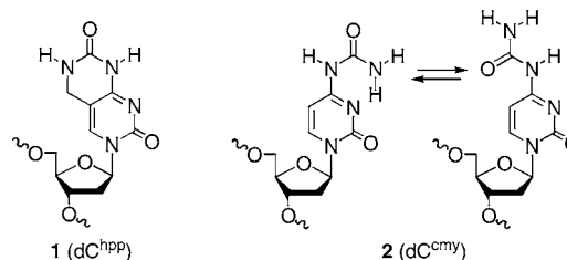
Figure 1. Chemical structures of dC hpp (1) and dC cmy (2) nucleosides.
