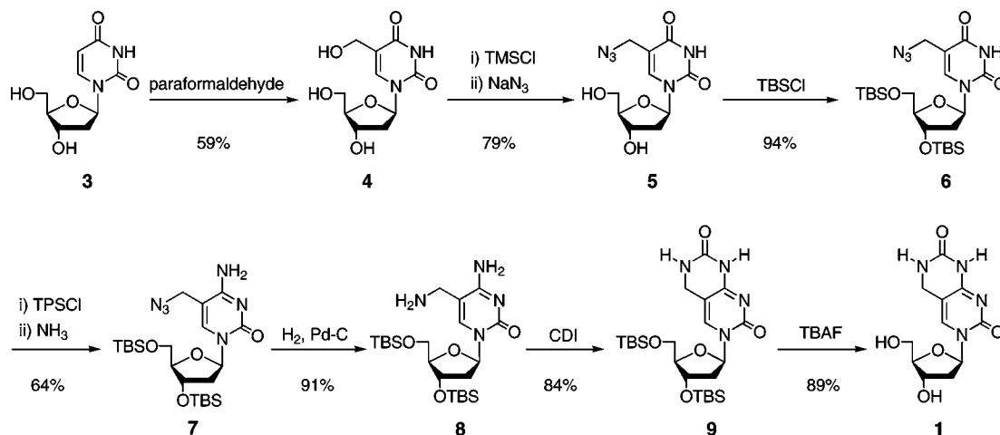
Scheme 1. Synthesis of Bicyclic 4- N -Carbamoyldeoxycytidine ( 1 , dC hpp )
