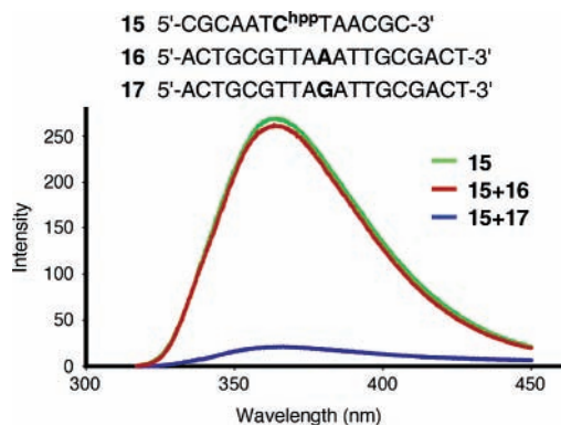
Figure 3. Fluorescent spectra of oligodeoxynucleotides containing dC hpp (5 \mu M nucleoside, 10 mM sodium phosphate, pH 7.0, excitation 300 nm).
