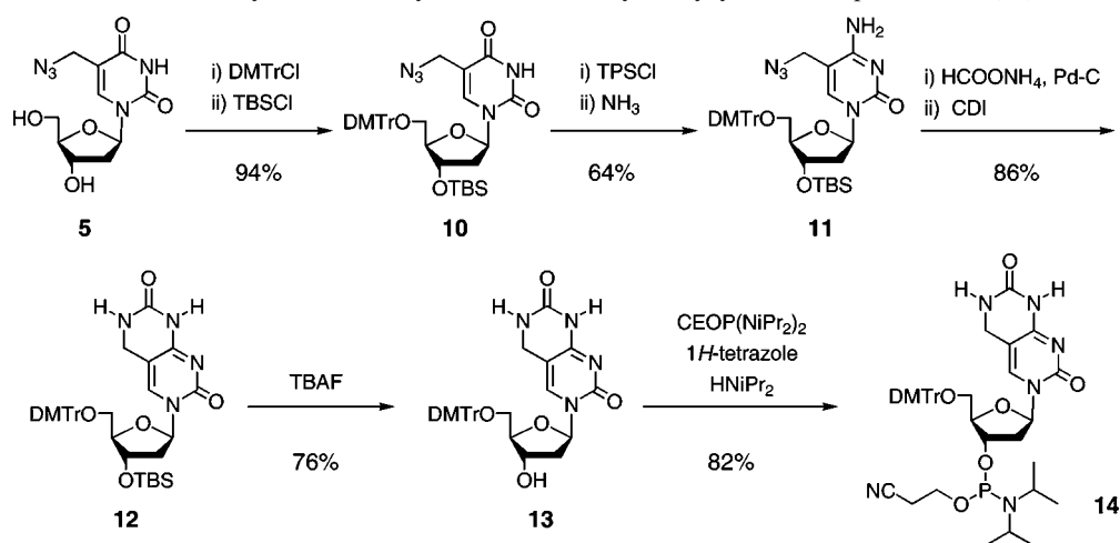
Scheme 2. Synthesis of Bicyclic 4- N -Carbamoyldeoxycytidine Phosphoramidite ( 14 )
