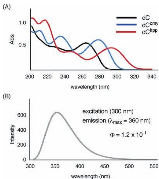
Figure 2. (A) UV absorption spectra of dC, dC cmv , and dC hpp : 80 \mu M nucleoside, 10 mM sodium phosphate, pH 7.0. (B) Fluorescent spectra of dC hpp : 5 \mu M nucleoside, 10 mM sodium phosphate, pH 7.0.
